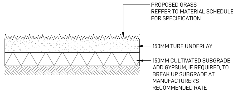
3 NATURAL TURF TYPICAL SECTION - SCALE 1:20
