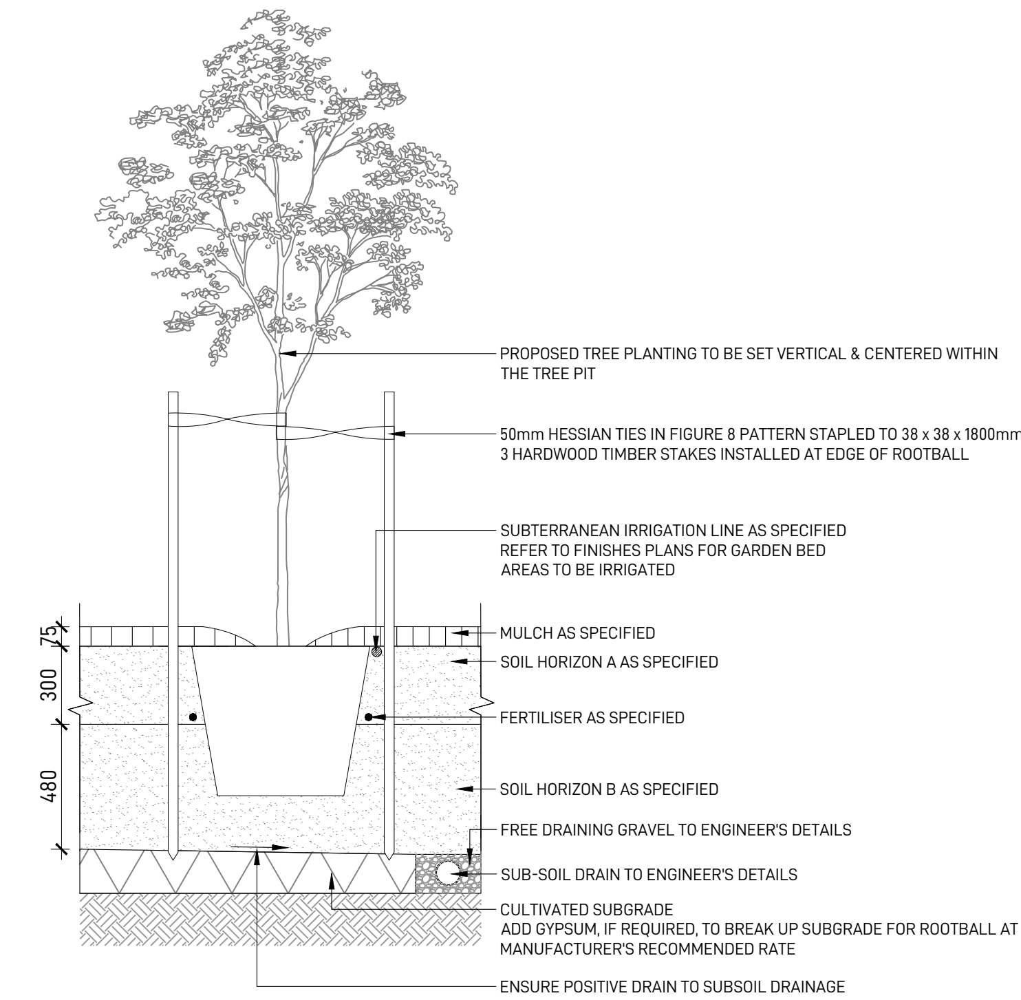
1 PLANTING - 100L TREE TYPICAL SECTION - SCALE 1:20
