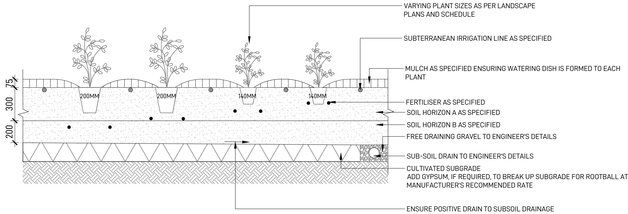
2 PLANTING - 200MM, 140MM TYPICAL SECTION - SCALE 1:20
